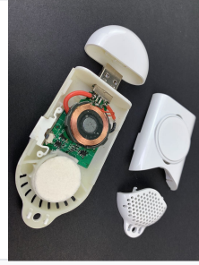
Internal components including the USB interface and electronic circuitry.
