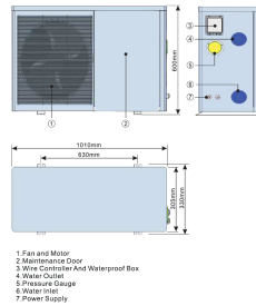
Dimensional drawing showing fan, motor, maintenance access, and water connection points.
