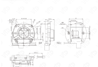
Technical drawing detailing the dimensions and specifications of the VIR29 optical module.
