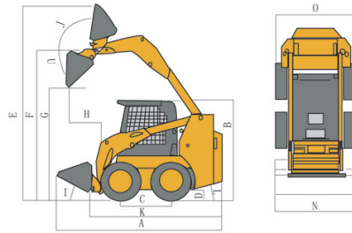
Engineering diagram showcasing dimensions and layout of the loader.
