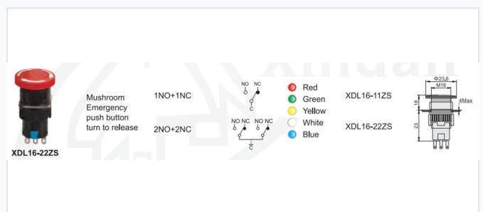
Dimension drawing showing the 23.6mm head and M16 mounting thread.
