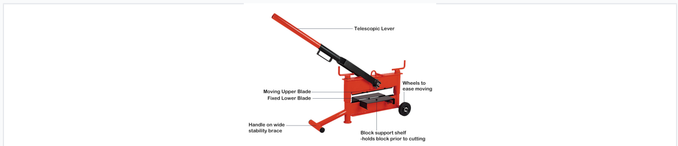
Detailed component overview of the manual paver block splitter, highlighting the telescopic lever, block support shelf, and mobility features.
