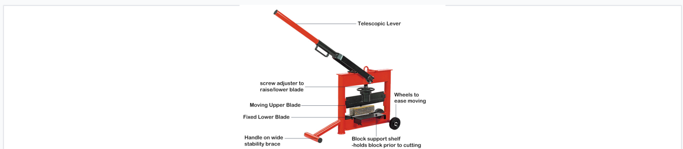
Detailed view of the splitter mechanism, featuring a telescopic lever for leverage, adjustable blade height, and a block support shelf for stability.
