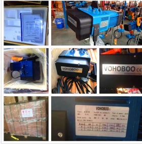
Technical data plate showing motor and performance specifications.
