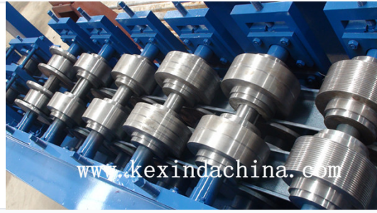
Complete production line including decoiler, forming stands, and run-out table.
