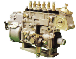
PW 3000 Pump Max Displacement 1.5 Liters/cylinder Max Output Power 45KW /cylinder Emission: Euro 1
