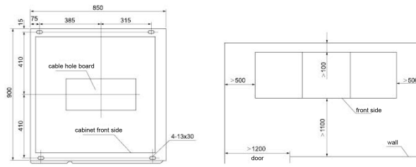
cabinet installation
