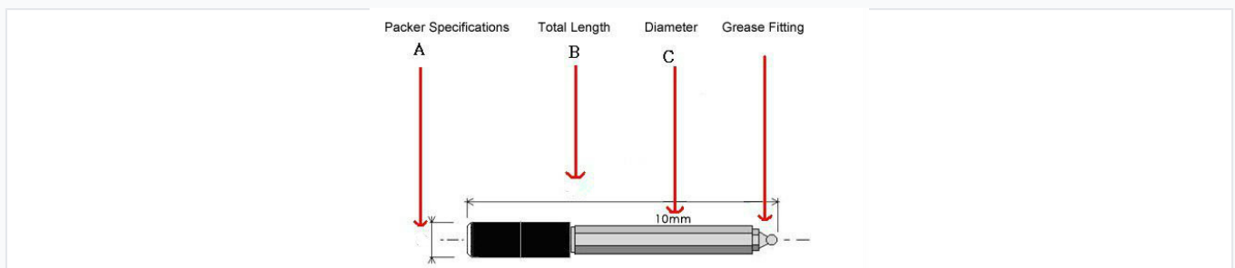
Detailed view of the mechanical injection packer featuring a grease fitting and 10mm diameter design.
