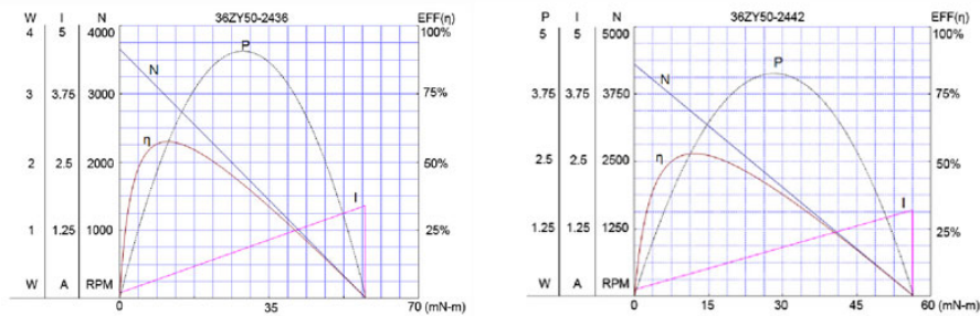
Speed, torque, current, and efficiency curves for the 2436 and 2442 motor variants.
