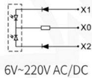
Double colour Metal Pilot light
